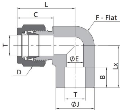
Fractional Tube to Tube Socket Weld
