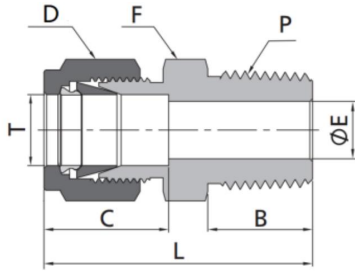
Fractional Tube to NPT Thread
