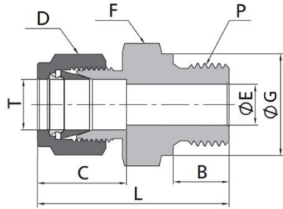
Fractional Tube to ISO Parallel Thread
