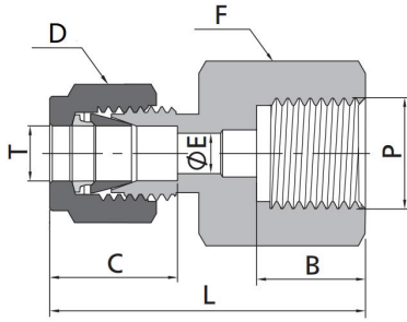
Fractional Tube to ISO Parallel Thread
