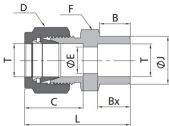
Fractional Tube to Tube Socket Weld
