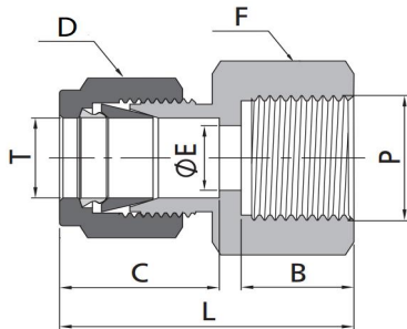
Fractional Tube to Metric Thread
