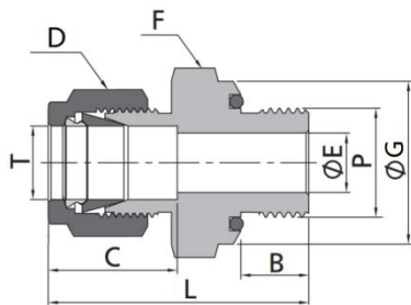
Fractional Tube to SAE/MS Thread
