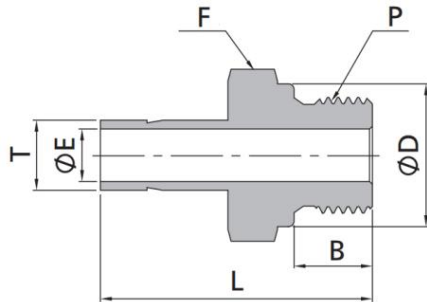
Fractional Tube to ISO Parallel Thread
